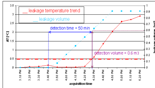
Fig.7. temperature and leaked volume evolution at leak location 3.
