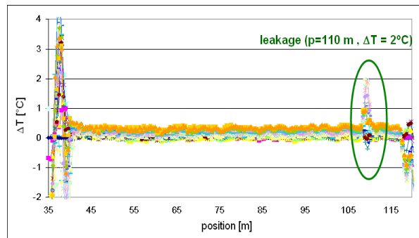
Fig.8. Relative temperature data for the leakage test.
