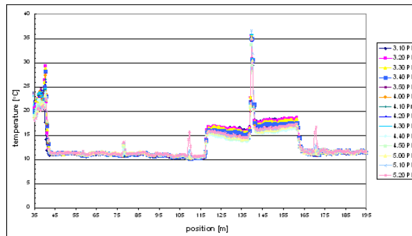
Fig.5. Raw temperature data for the leakage test.
