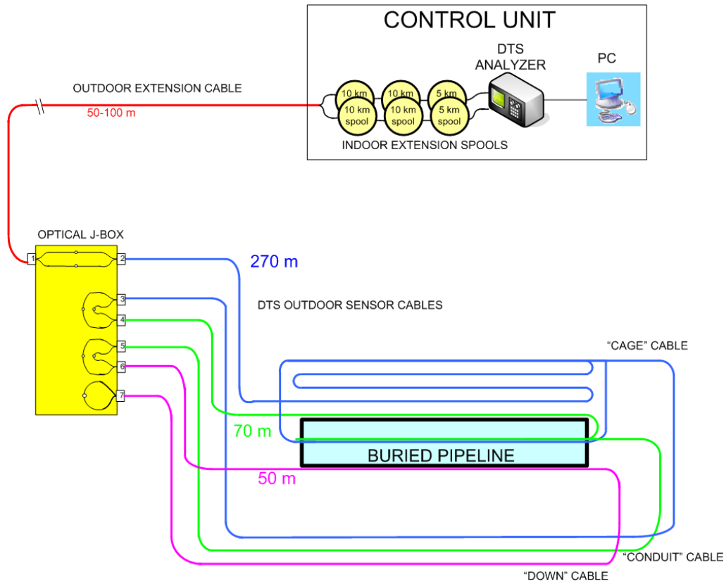
Fig.16. Test setup.
