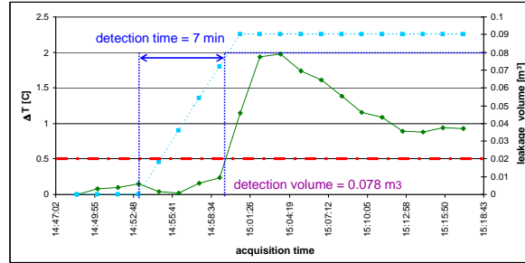
Fig.9. Temperature and leaked volume evolution at leak location D5, 2nd test with \Delta T=3^{\circ}\text{C} .
