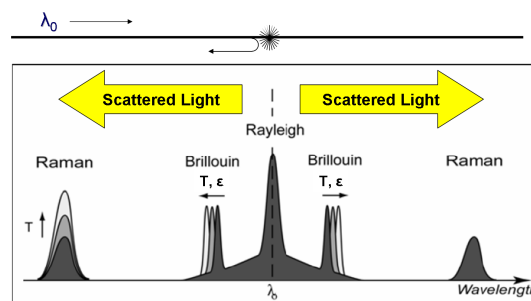
Fig.1. Light scattering in optical fiber.
