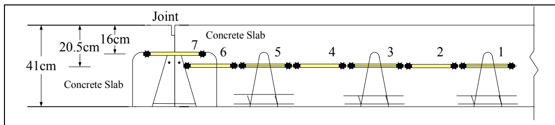
Figure 2. Cross View of Optical Fiber Sensors Installation.
