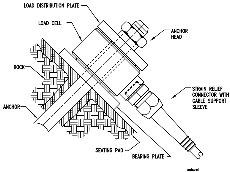
Figure 2: VH typical installation on a tie-back
