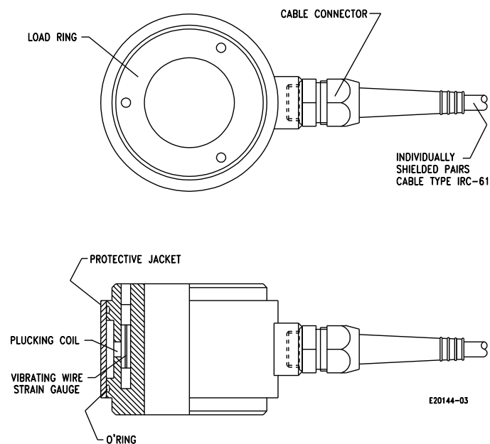
Figure 1: VH Load Cell, model with 3 strain gauges and a hollow center
