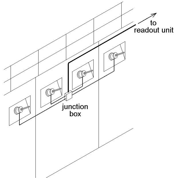
Figure 3: Example of junction box use
